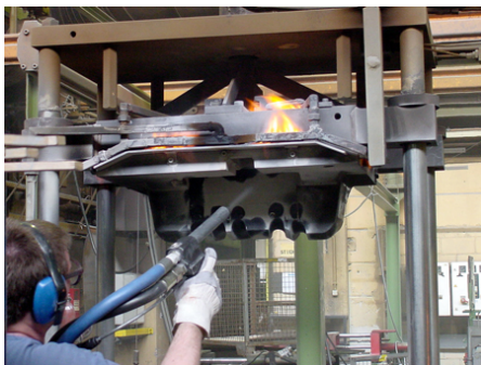
Figure 2 – Efficient online cleaning of a hot ingot mould.
